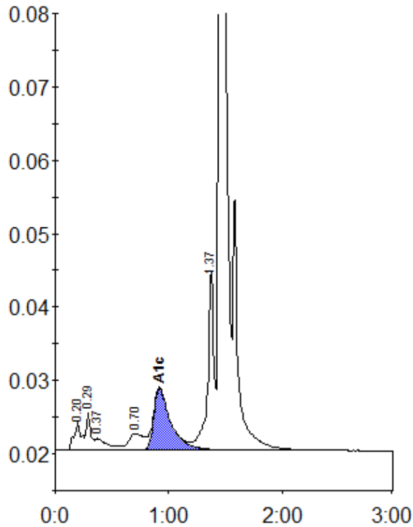
Peak table - ID: 10348031
